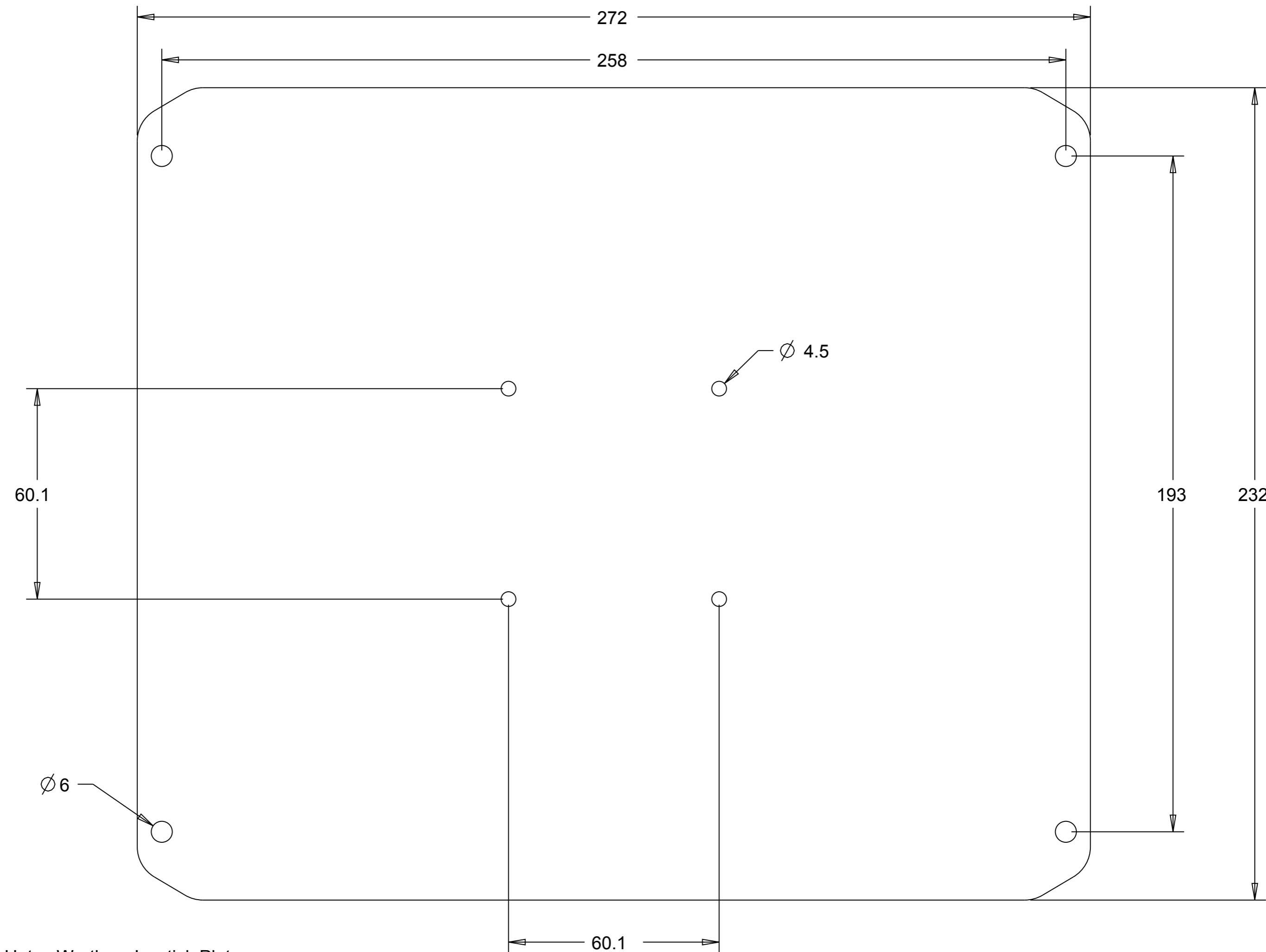
Hotas Warthog Joystick Plate Dimensions in mm
